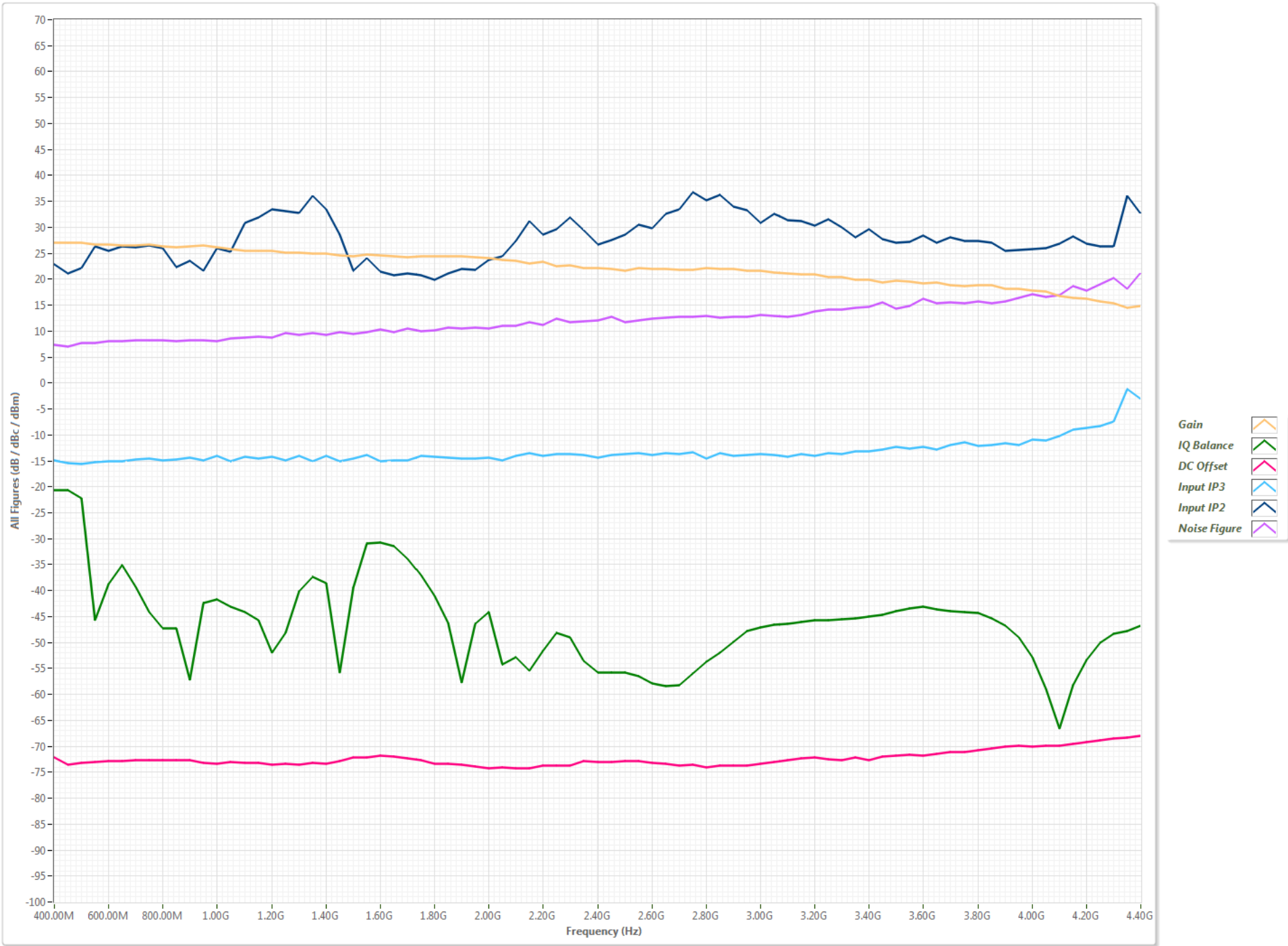
RX Figure vs Frequency w/ Gain=25.00dB
