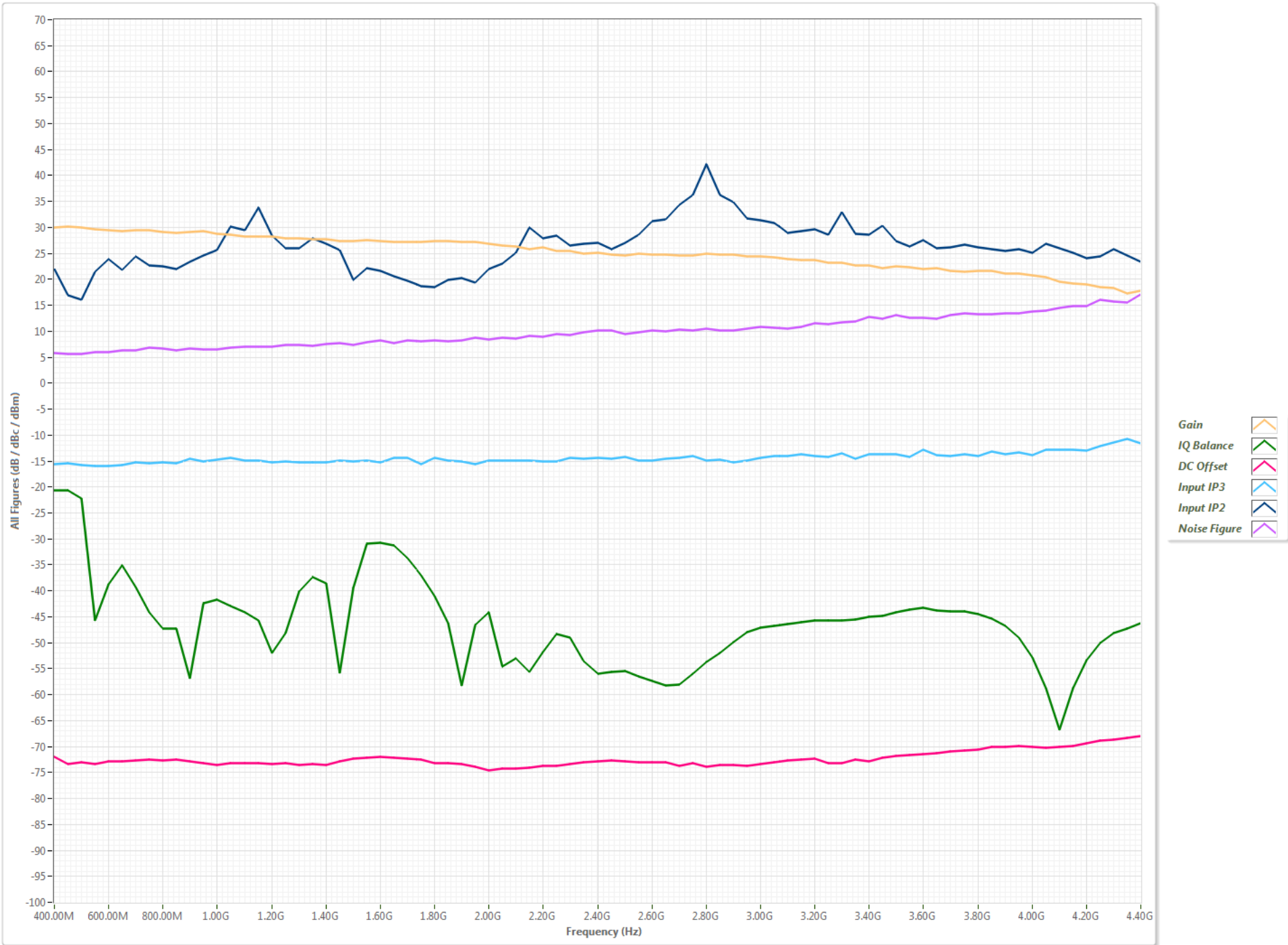
RX Figure vs Frequency w/ Gain=28.00dB
