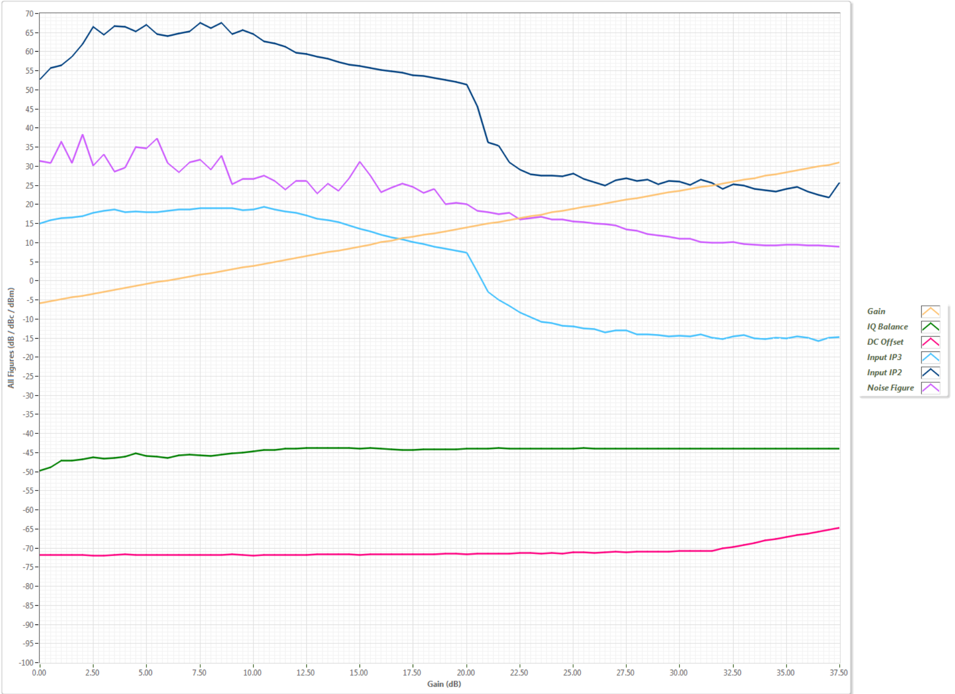
RX Figure vs Gain w/ Frequency=3700.00MHz
