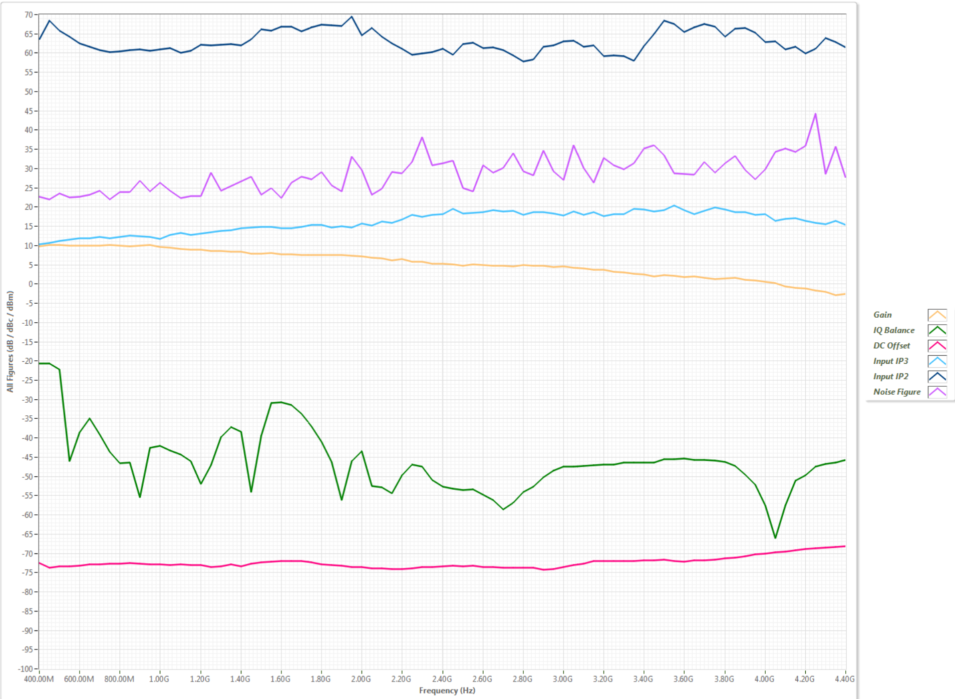
RX Figure vs Frequency w/ Gain=7.50dB
