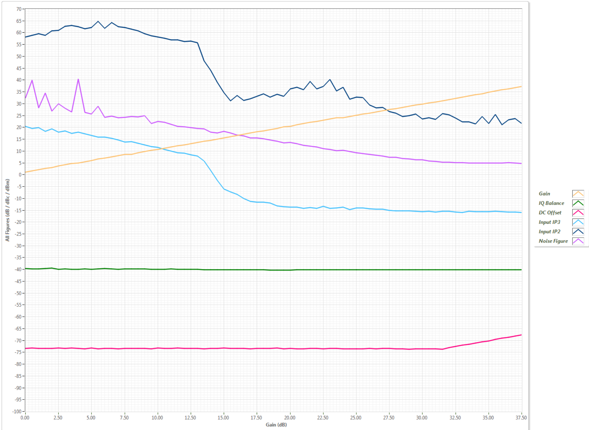
RX Figure vs Gain w/ Frequency=1300.00MHz
