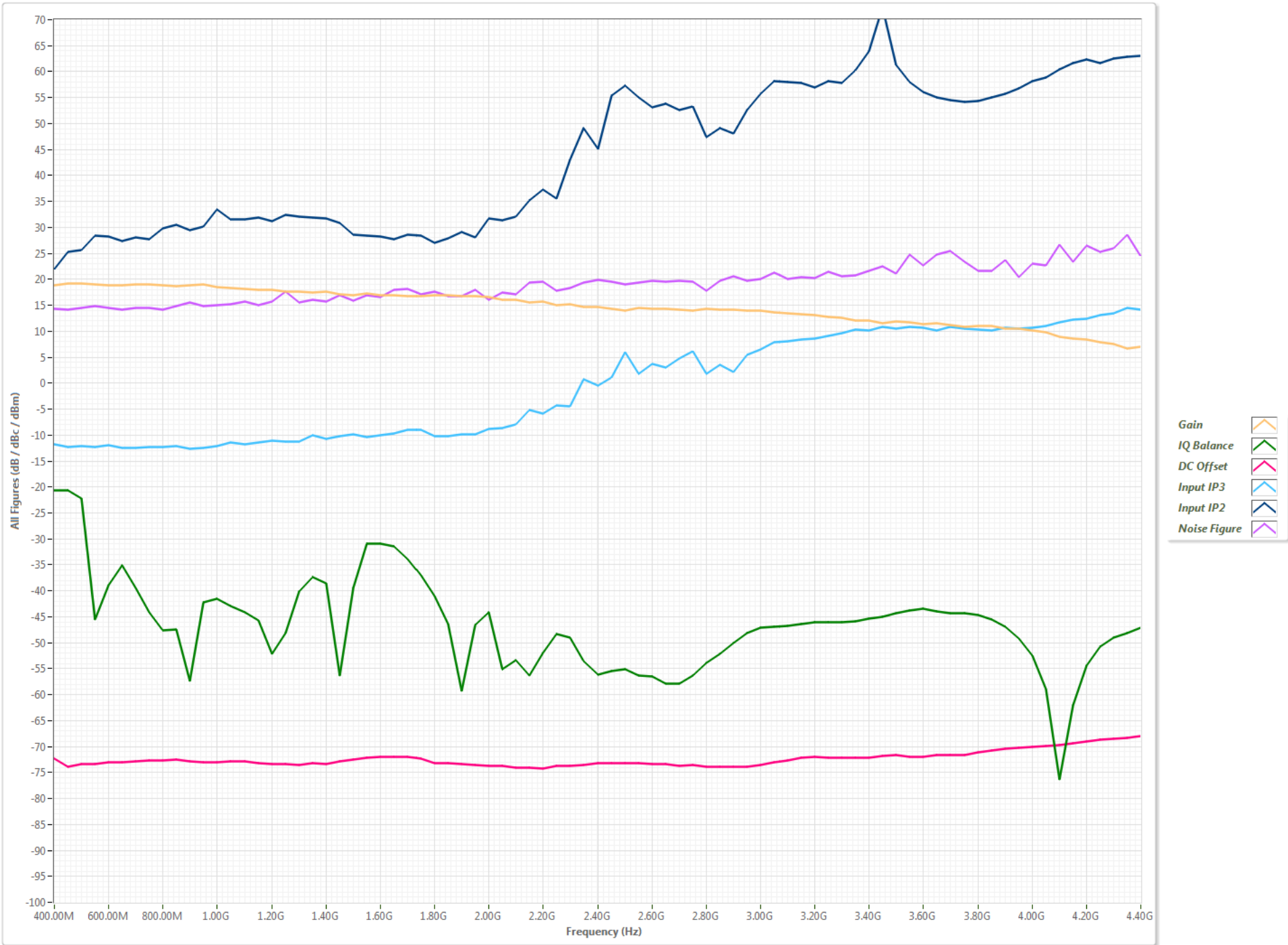
RX Figure vs Frequency w/ Gain=17.00dB
