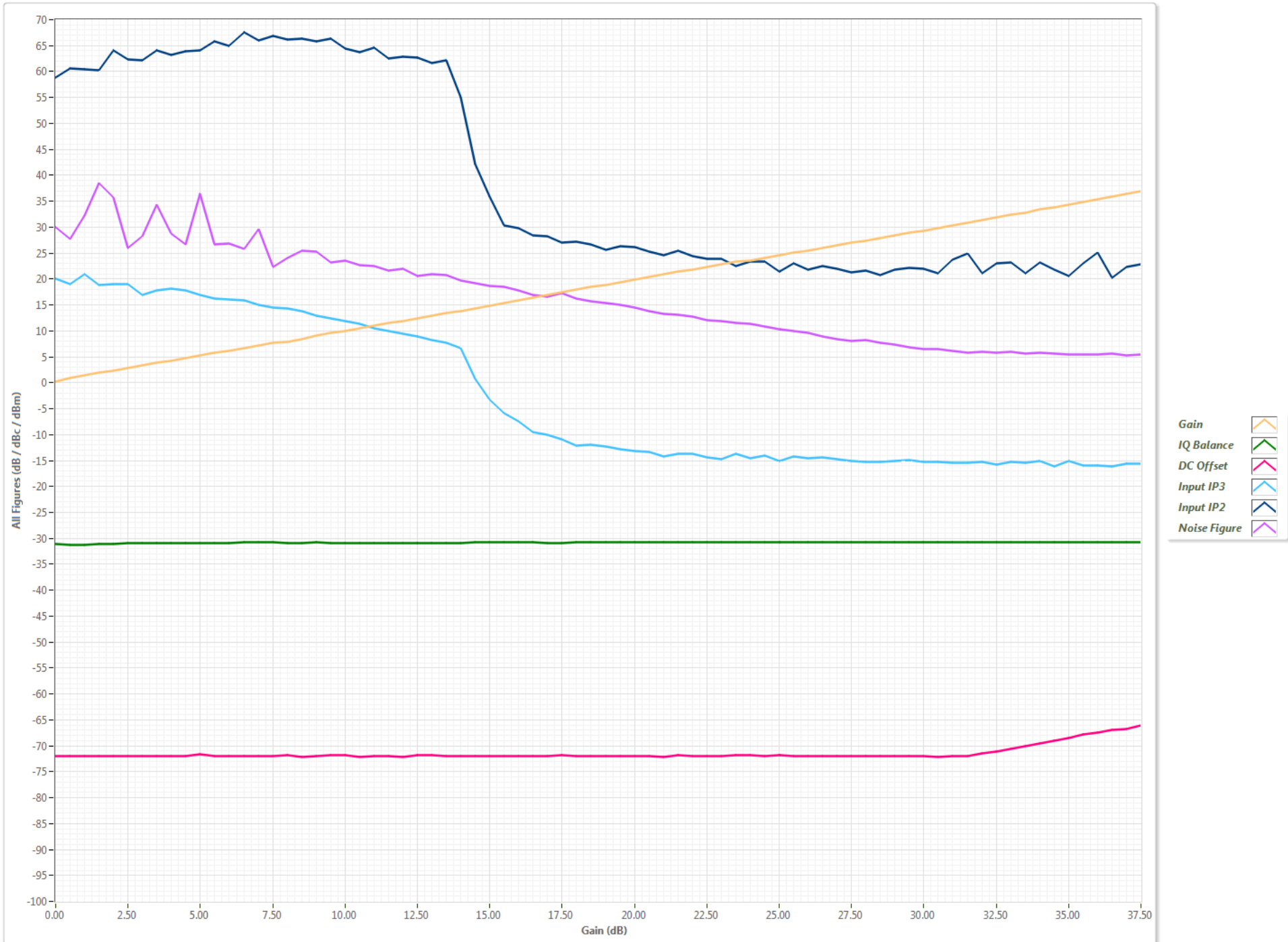
RX Figure vs Gain w/ Frequency=1600.00MHz
