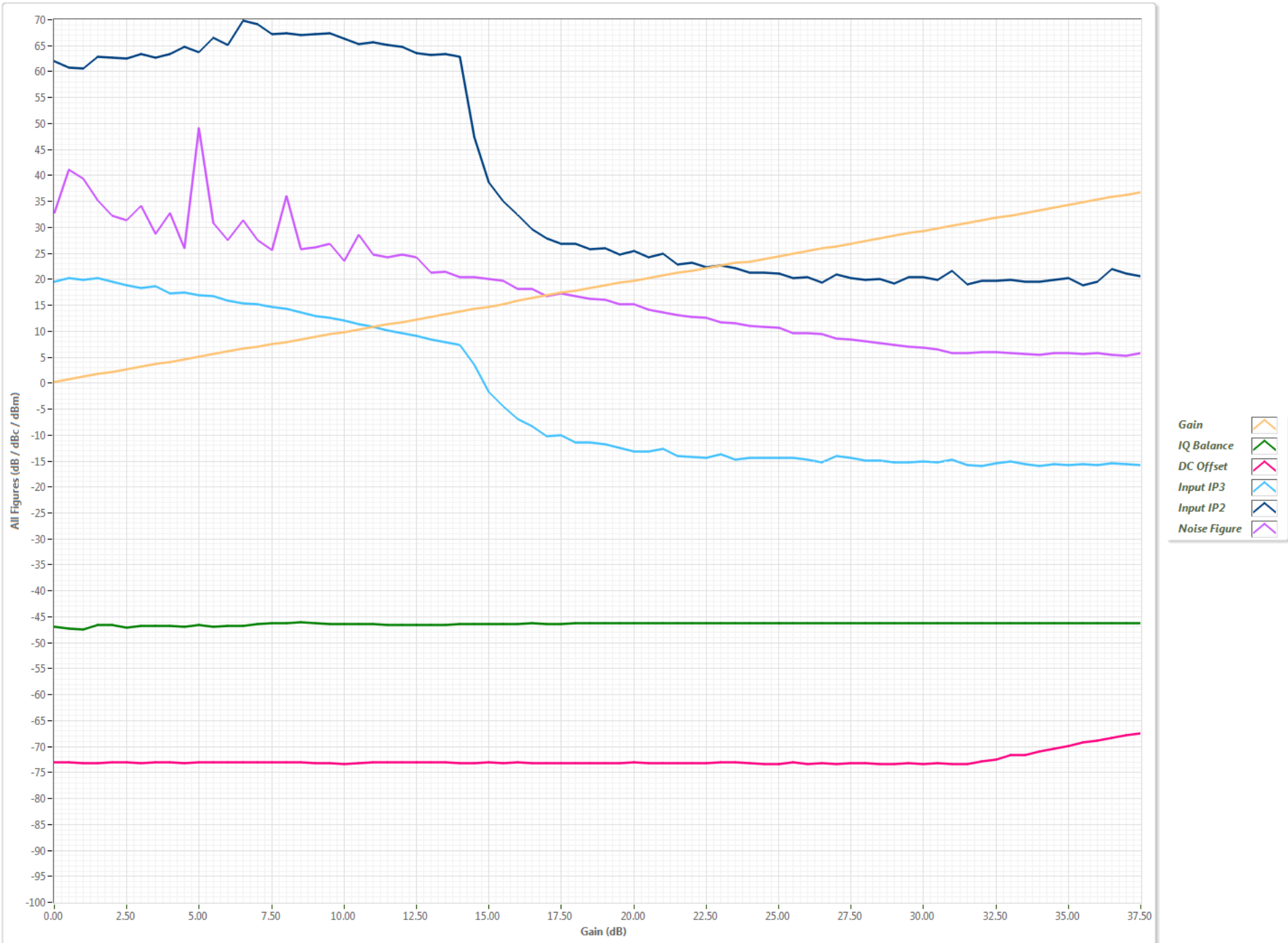
RX Figure vs Gain w/ Frequency=1850.00MHz
