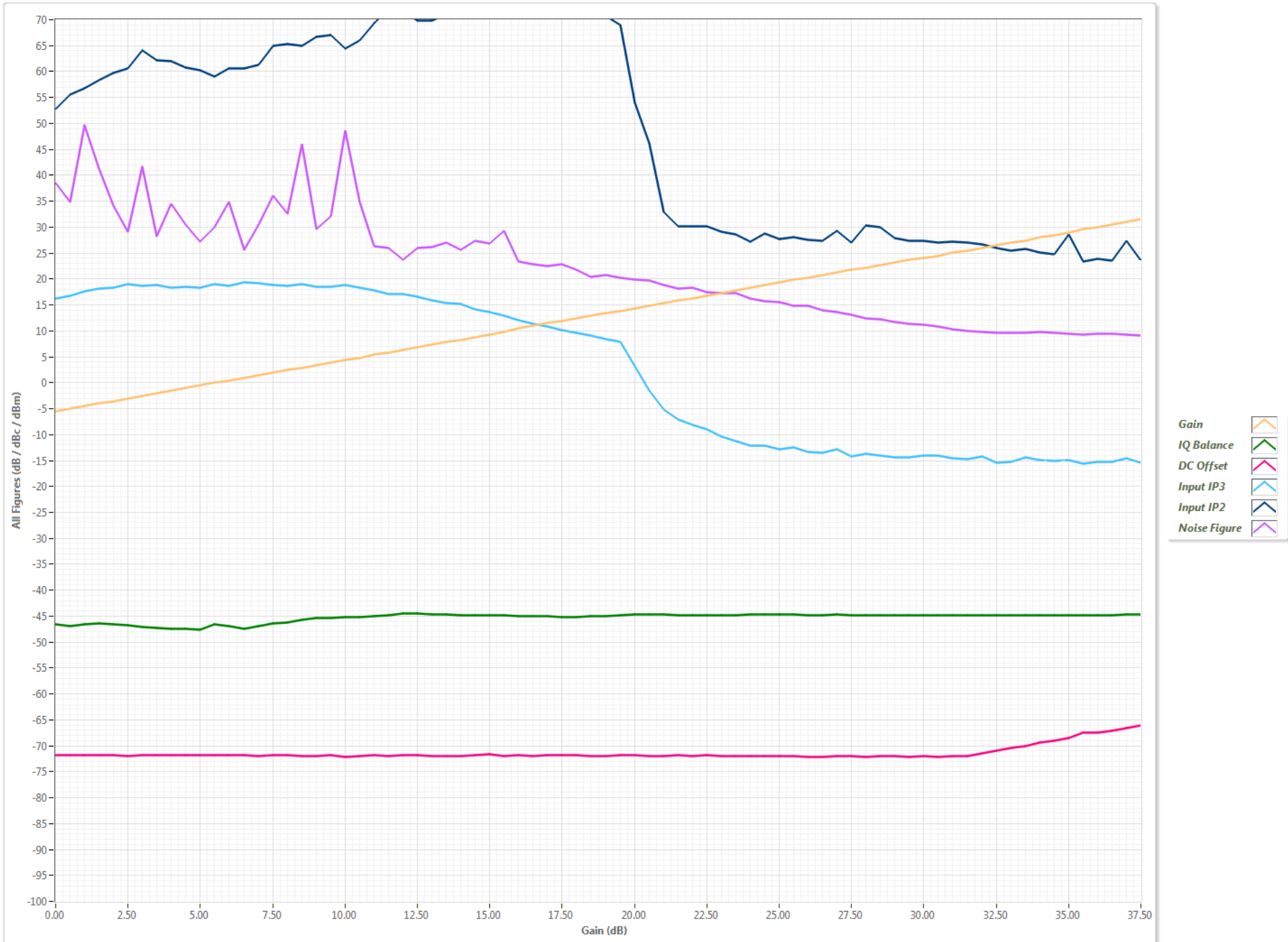
RX Figure vs Gain w/ Frequency=3450.00MHz
