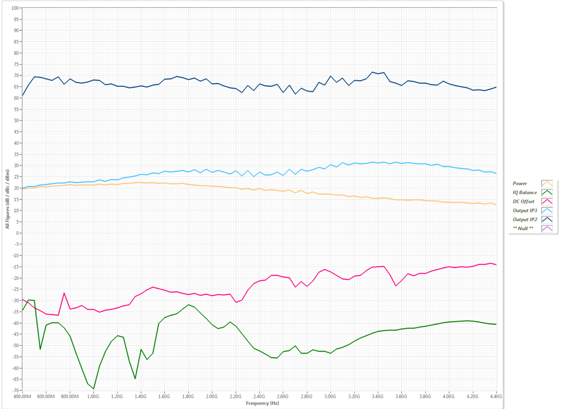
TX Figure vs Frequency w/ Gain=26.00dB
