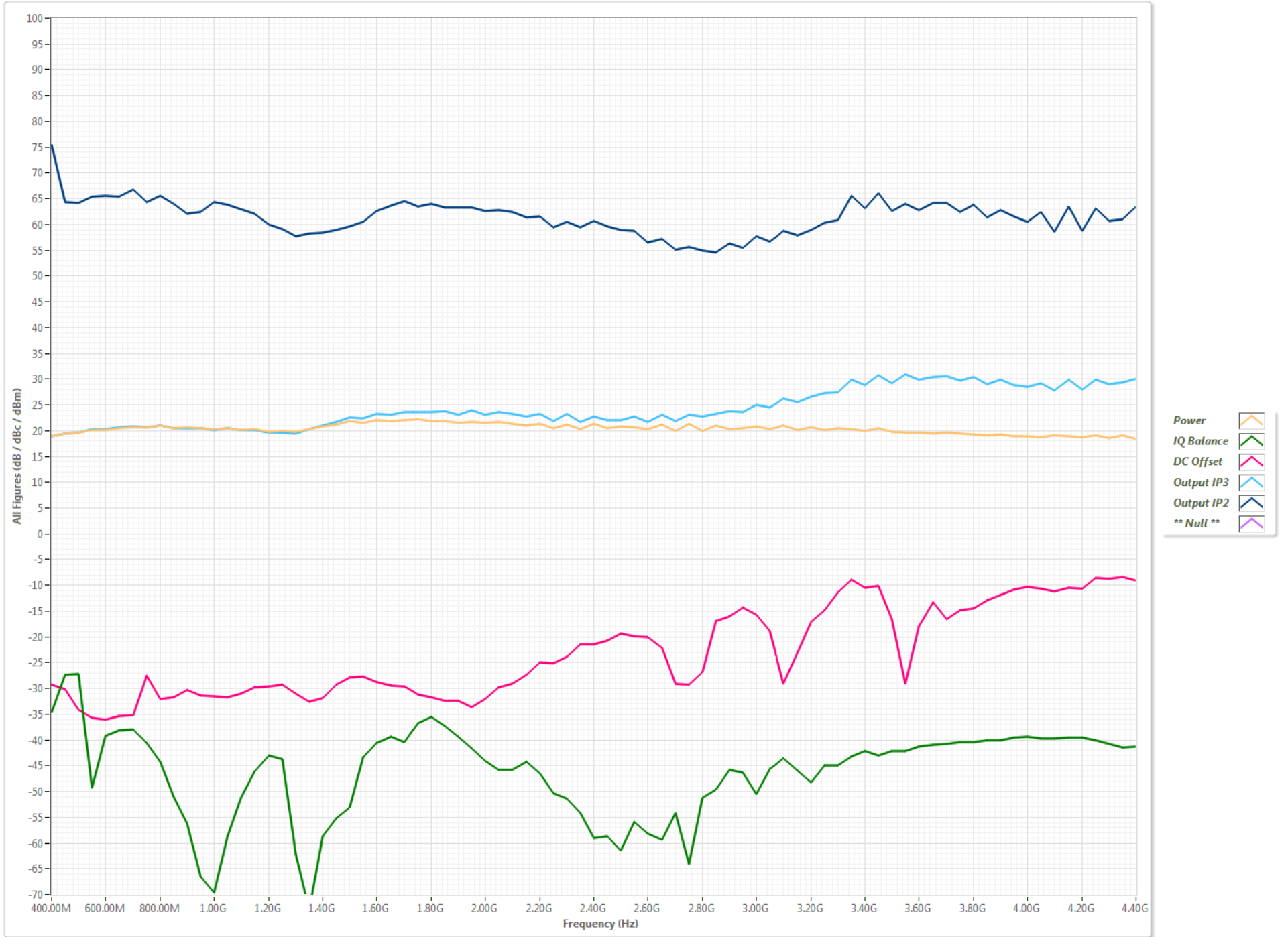
TX Figure vs Frequency w/ Gain=32.00dB
