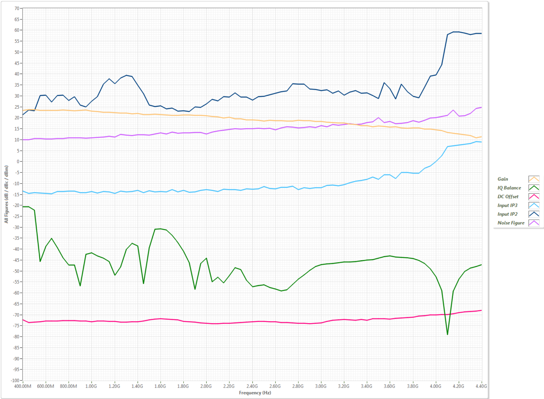
RX Figure vs Frequency w/ Gain=21.50dB
