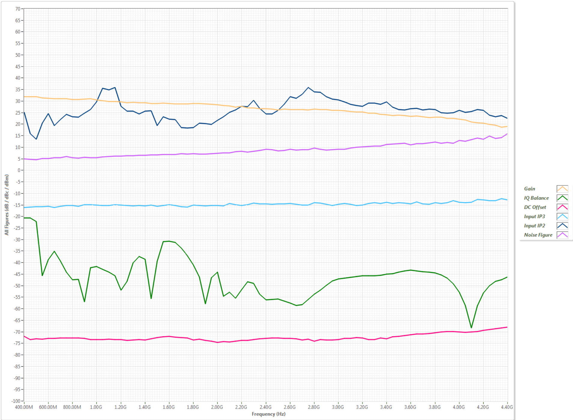
RX Figure vs Frequency w/ Gain=29.50dB
