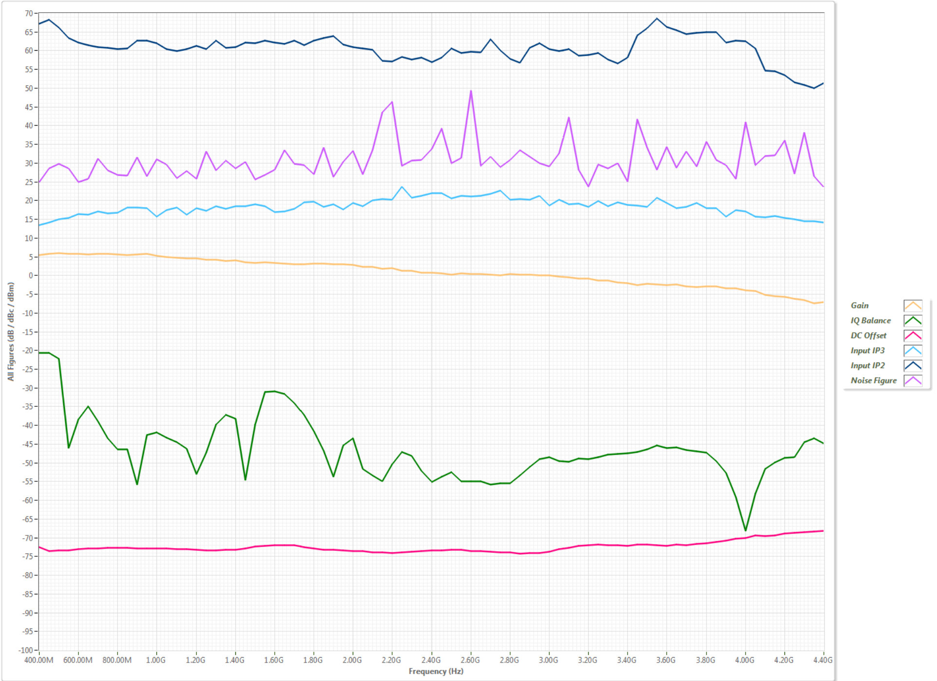
RX Figure vs Frequency w/ Gain=3.00dB
