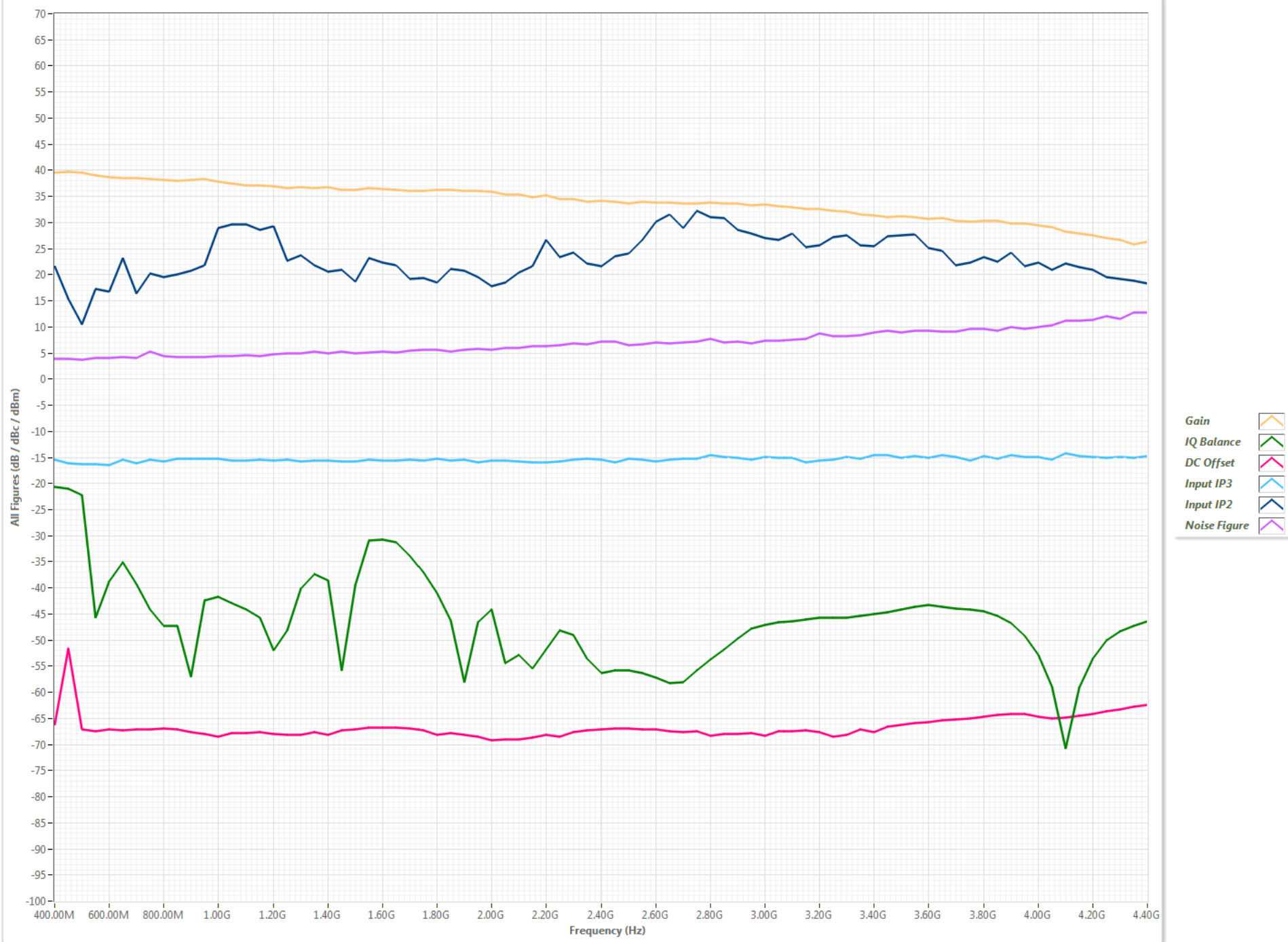
RX Figure vs Frequency w/ Gain=37.00dB
