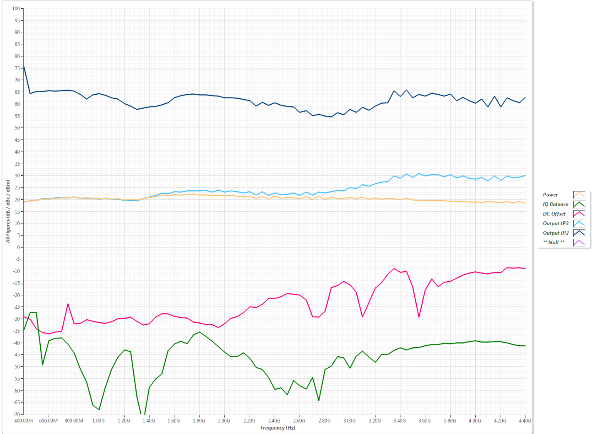
TX Figure vs Frequency w/ Gain=36.00dB
