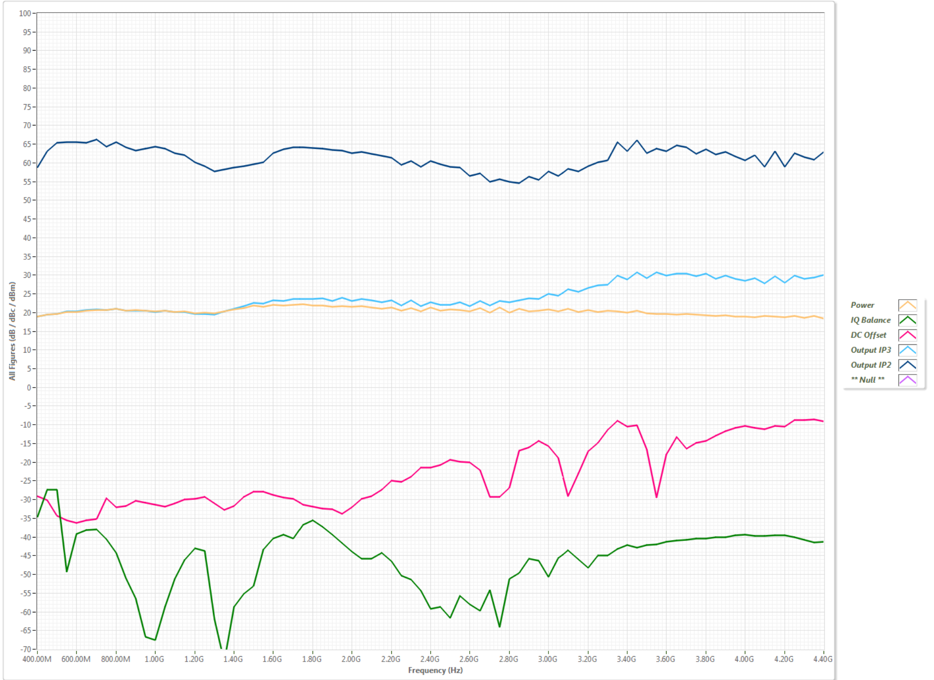
TX Figure vs Frequency w/ Gain=34.50dB
