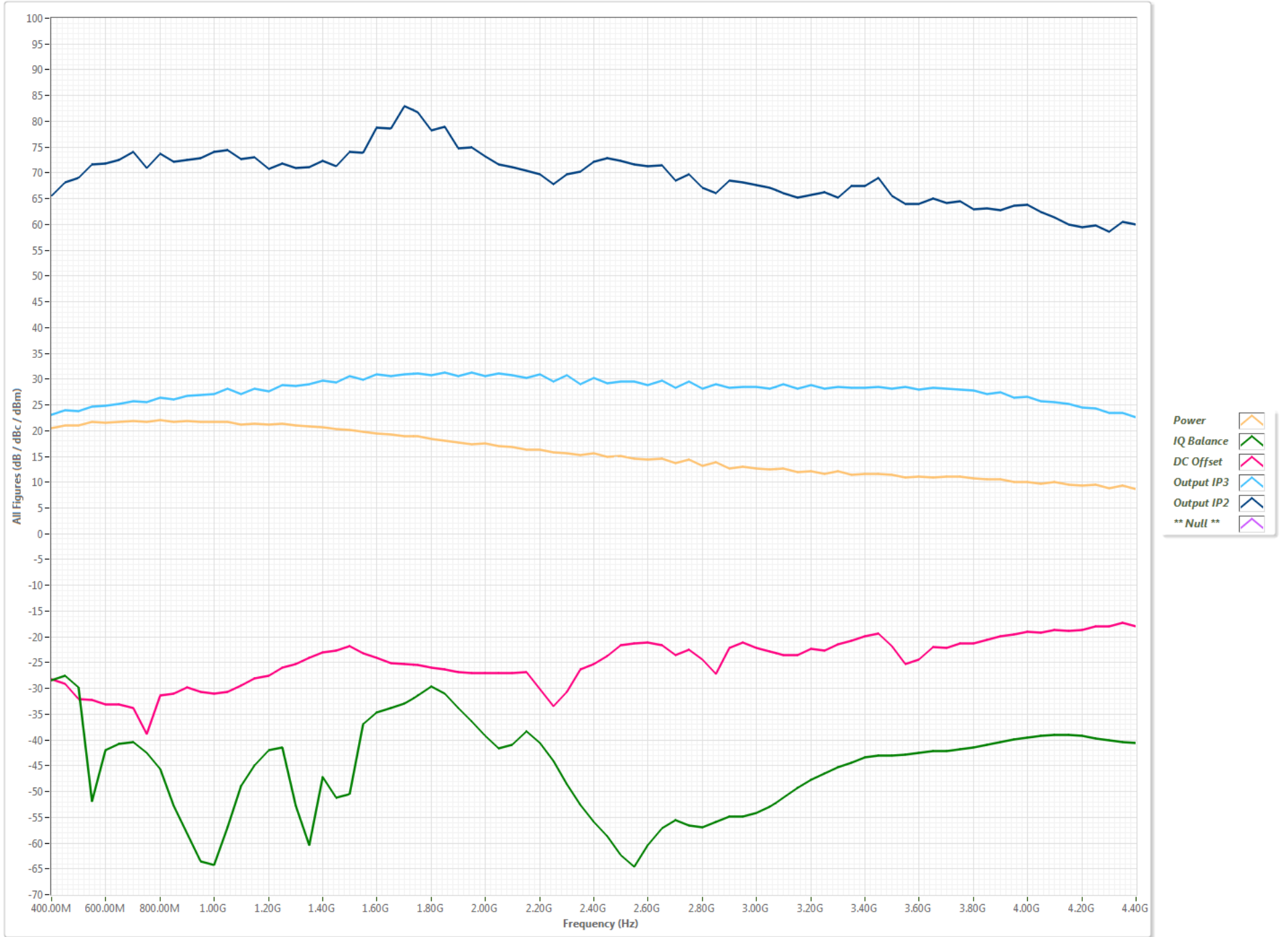
TX Figure vs Frequency w/ Gain=21.50dB
