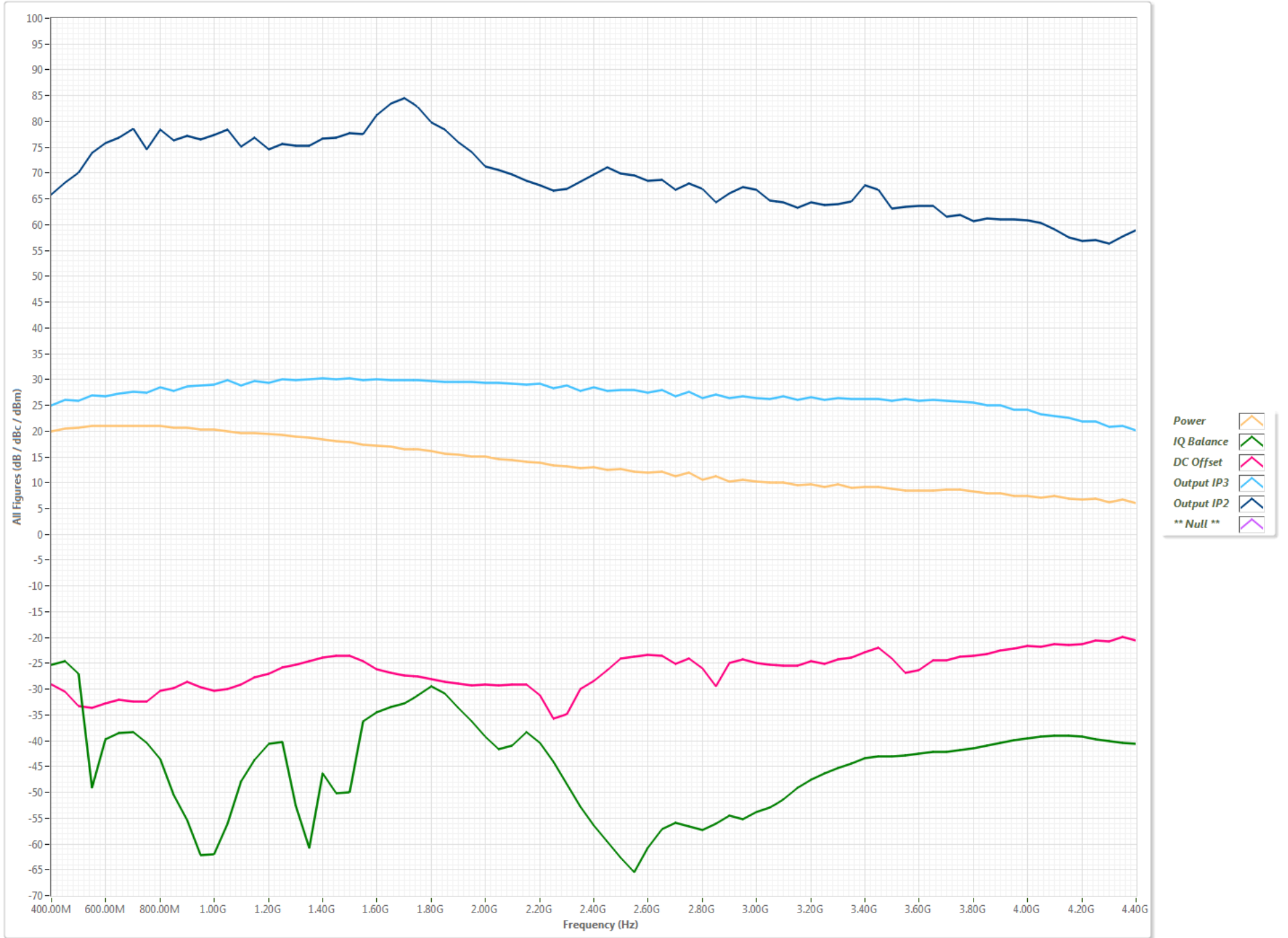
TX Figure vs Frequency w/ Gain=19.00dB
