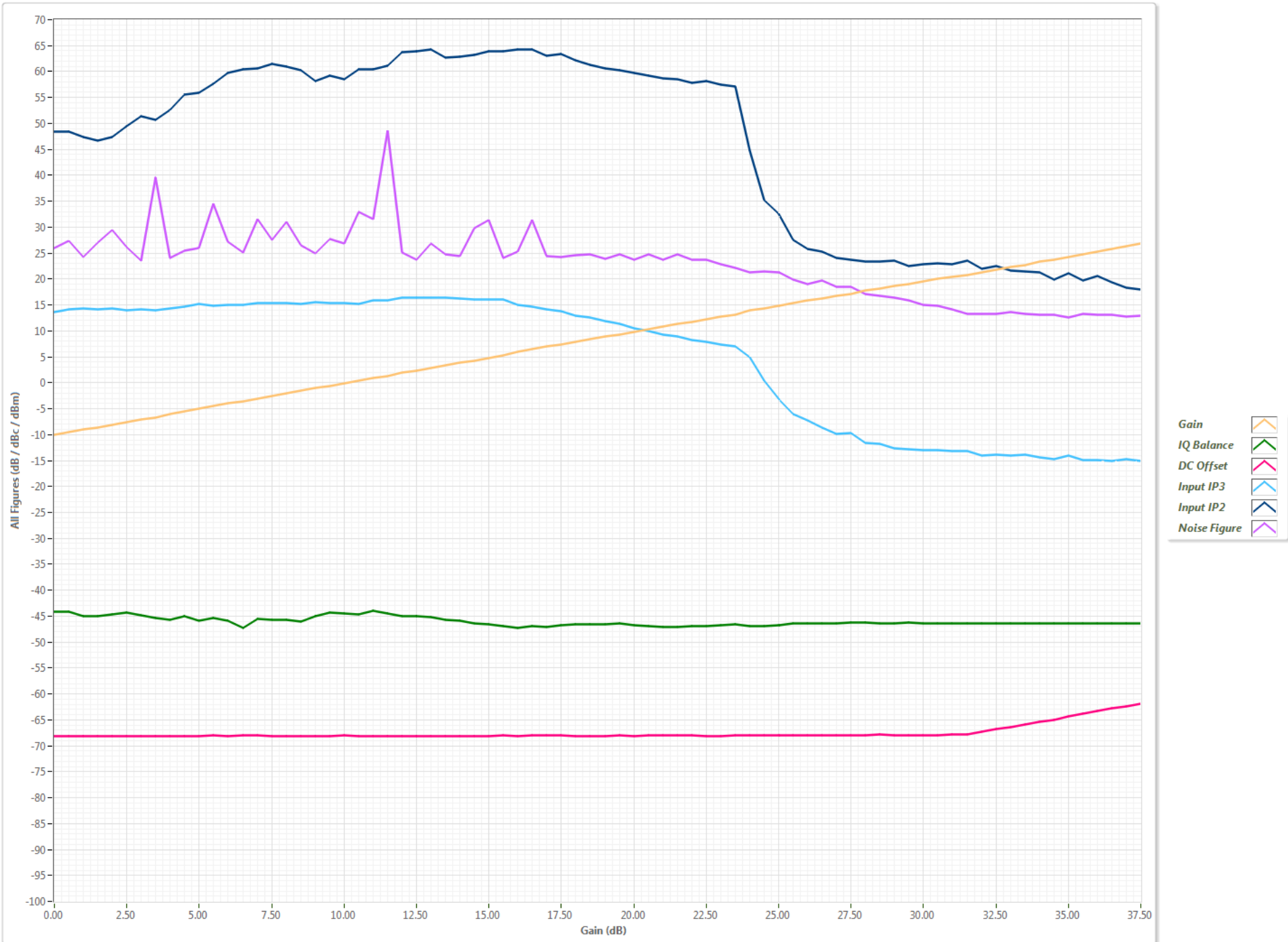
RX Figure vs Gain w/ Frequency=4400.00MHz
