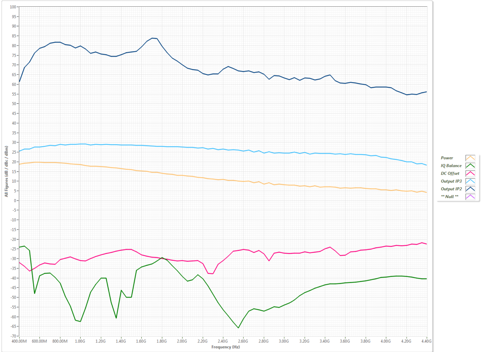
TX Figure vs Frequency w/ Gain=17.00dB
