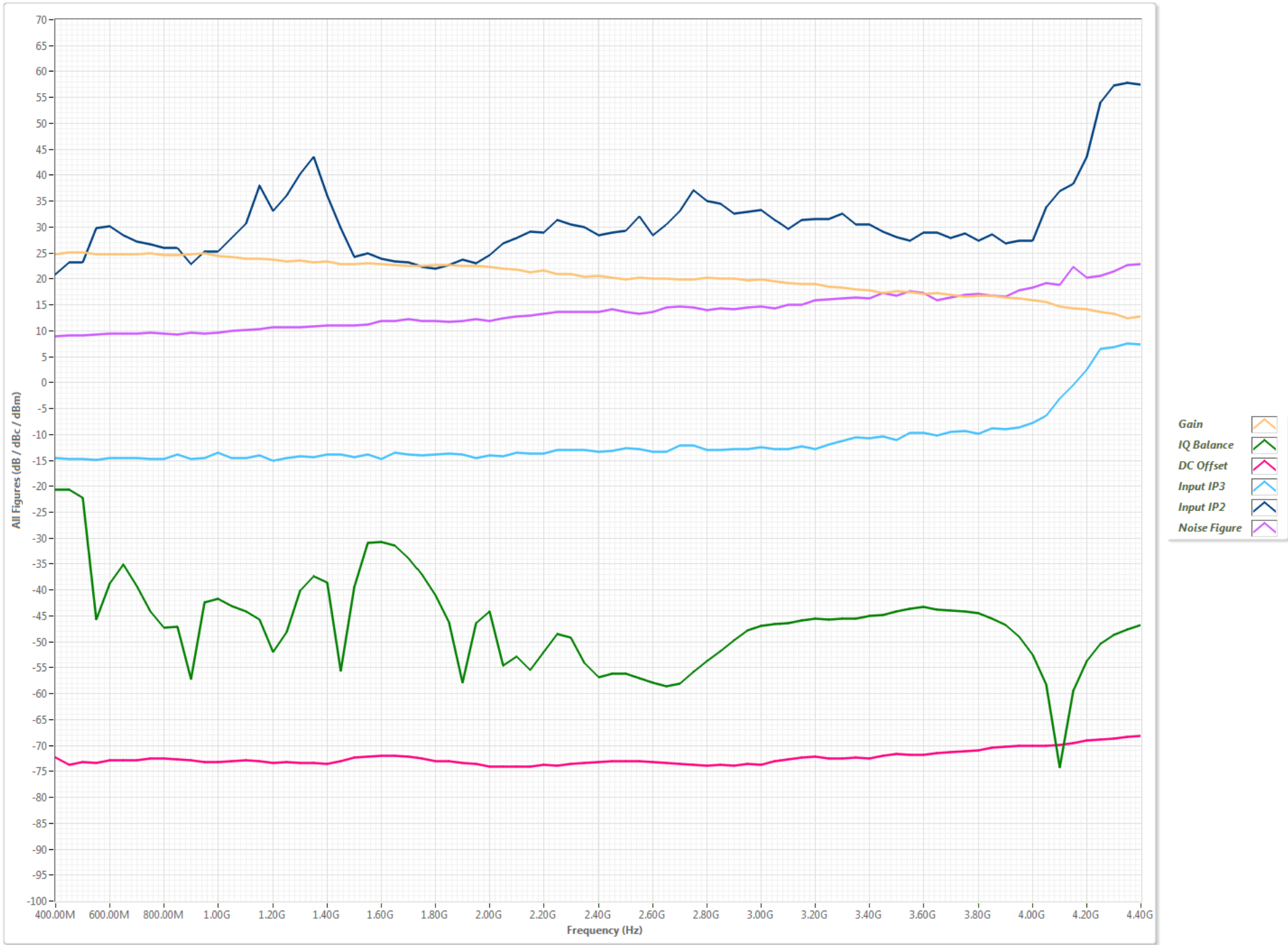
RX Figure vs Frequency w/ Gain=23.00dB
