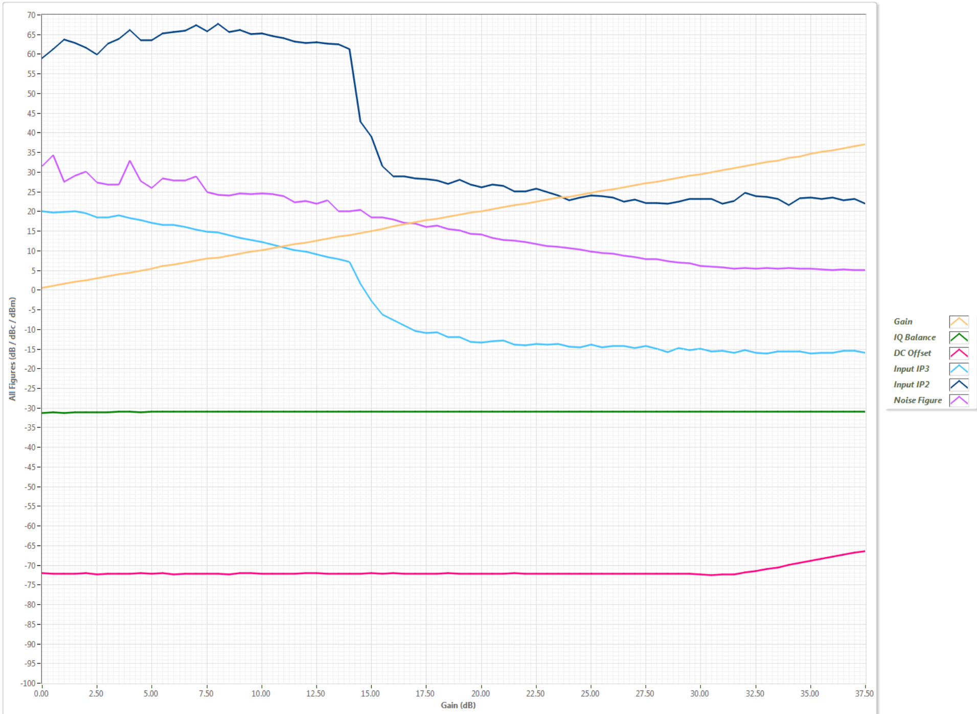
RX Figure vs Gain w/ Frequency=1550.00MHz
