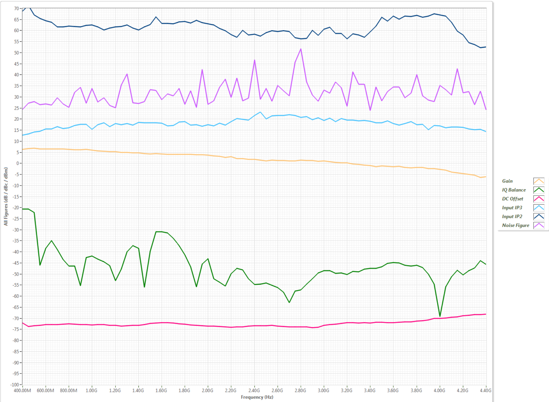
RX Figure vs Frequency w/ Gain=4.00dB
