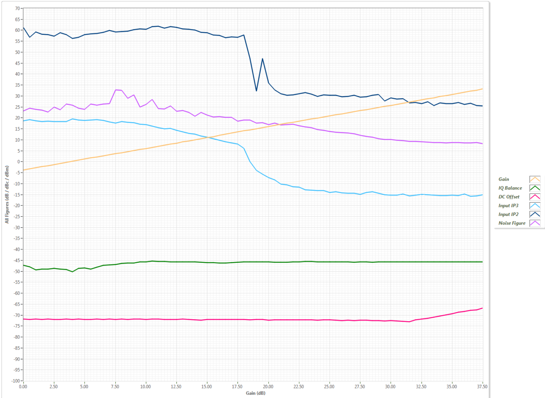
RX Figure vs Gain w/ Frequency=3200.00MHz
