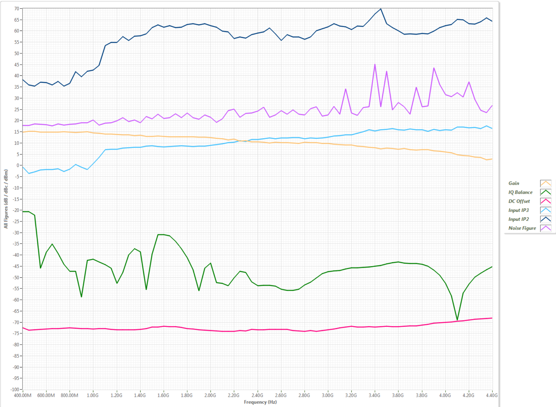
RX Figure vs Frequency w/ Gain=13.00dB
