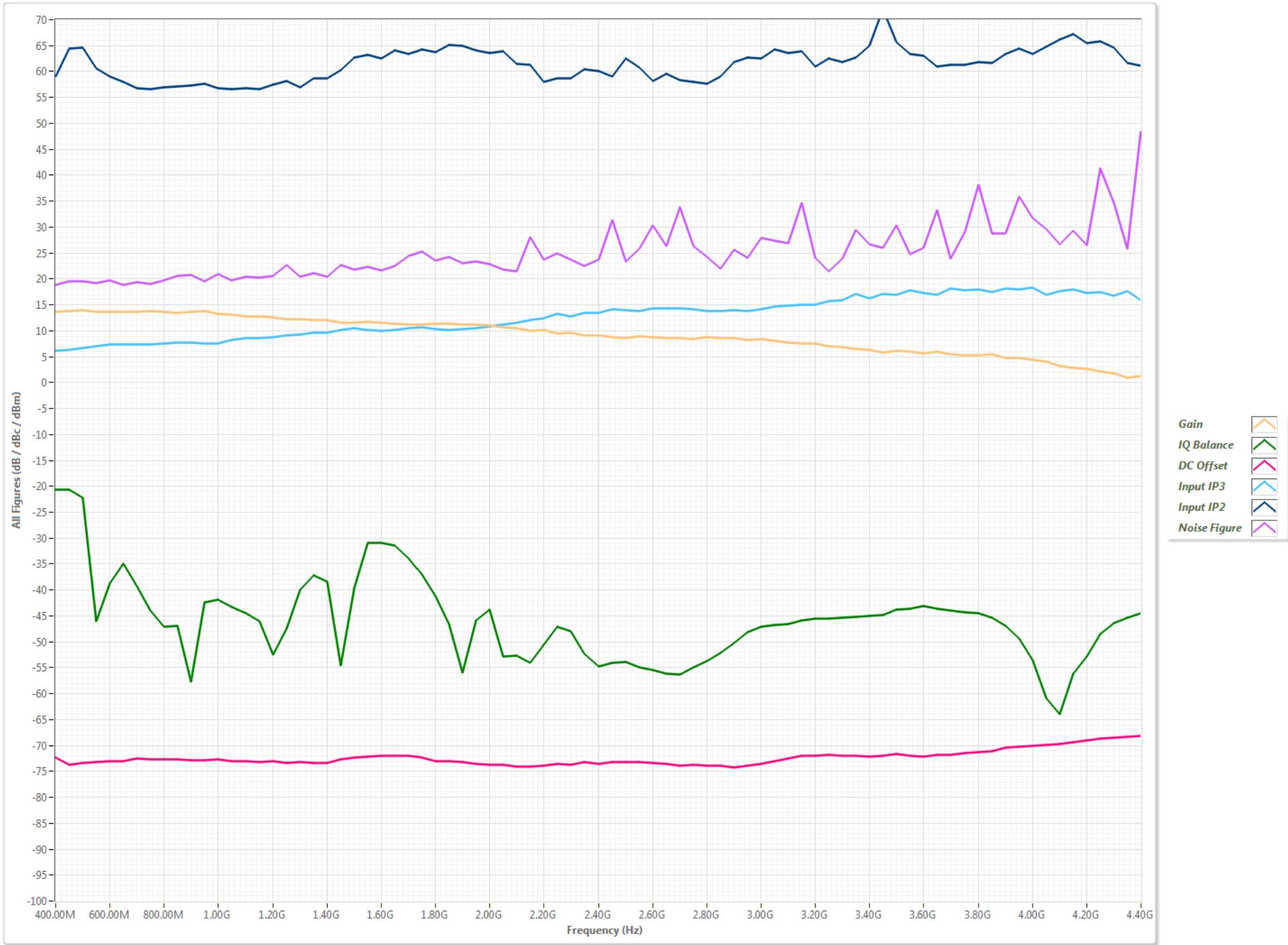
RX Figure vs Frequency w/ Gain=11.50dB
